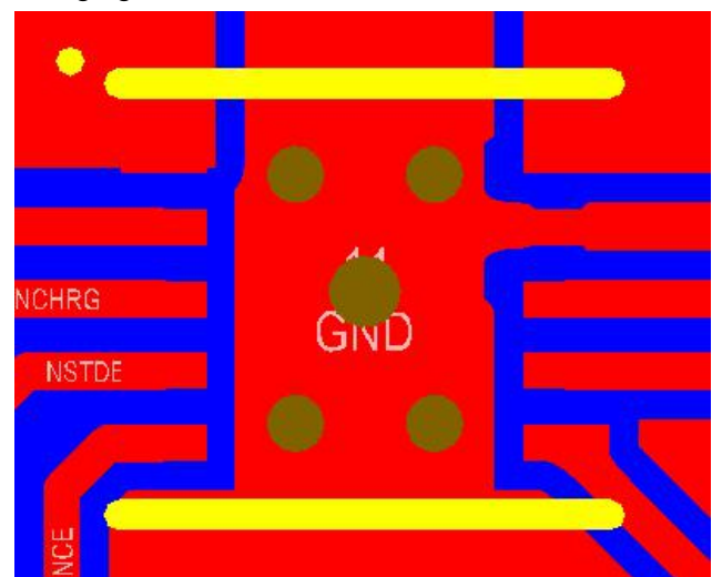
Figure 5 PCB layout
