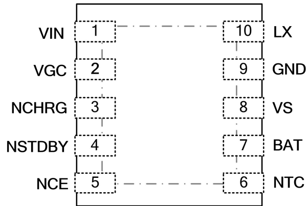
Figure 4. SLM6305 Pin package
